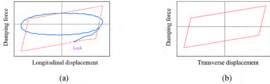
Fig. 2. The force-displacement relationship of HBHDS in the (a) longitudinal direction and (b) transverse direction.
