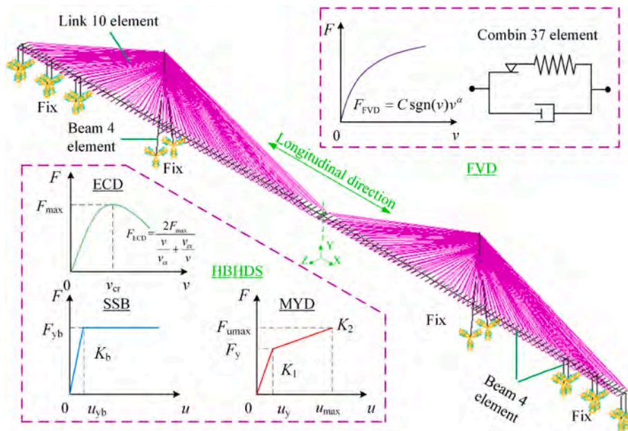
Fig. 4. Configuration and finite element model of the long-span bridge.
