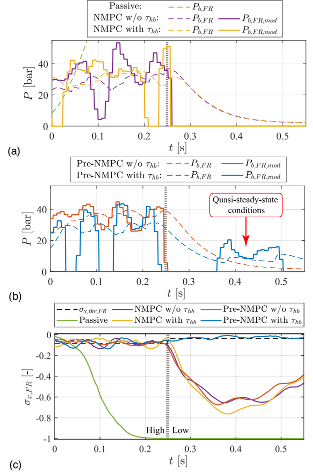
Fig. 15. Experimental test results along the high-to-low friction ABS test from 40 km/h: (a) P_{b,FR} and P_{b,FR,mod} profiles for “Passive”, “NMPC w/o \tau_{hb} ”, and “NMPC with \tau_{hb} ”; (b) P_{b,FR} and P_{b,FR,mod} profiles for “Pre-NMPC w/o \tau_{hb} ”, and “Pre-NMPC with \tau_{hb} ”; and (c) \sigma_{x,FR} profiles for all configurations, together with the corresponding \sigma_{x,thr,FR} time plot.
