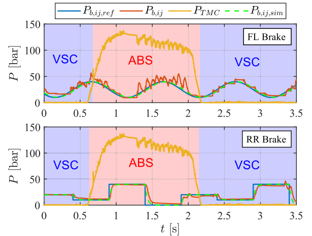
Fig. 6. Experimental results of the low-level feedback controller for the primary brake circuit.
