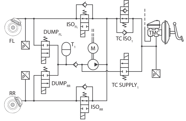
Fig. 3. Hydraulic schematic of the primary circuit of the modified VSC unit, serving the front left (FL) and rear right (RR) calipers. Pressure sensors are installed at the brake calipers and TMC.
