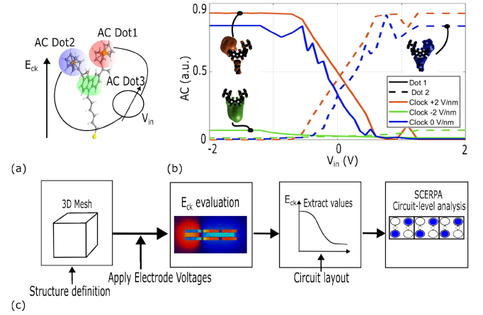
Fig. 2. (a) Schematic definition of V_{in} and the AC. (b) VACTs of the bis-ferrocene cation under E_{ck} = +2 V/nm, E_{ck} = -2 V/nm and E_{ck} = 0 V/nm. (c) Schematic flow diagram proposed in this work. The device mesh is calculated, and V_{el} are applied to extract the electric fields used for propagation analysis in SCERPA.
