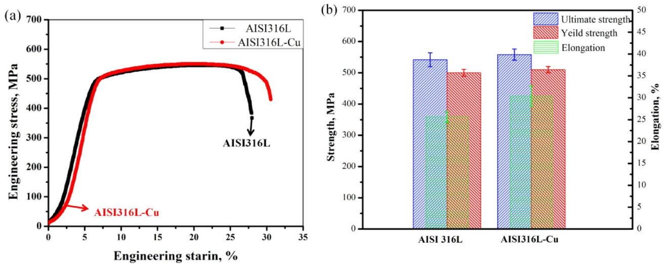
Fig. 7 a Engineering stress–strain curves and b results of tensile test of the as-built AISI316L and AISI316L-Cu samples
