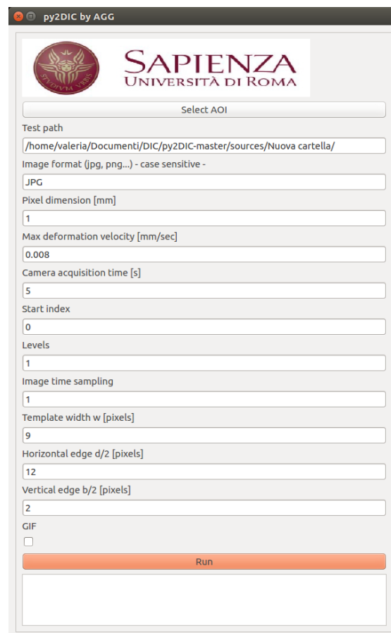
Figure 1. py2DIC GUI.
