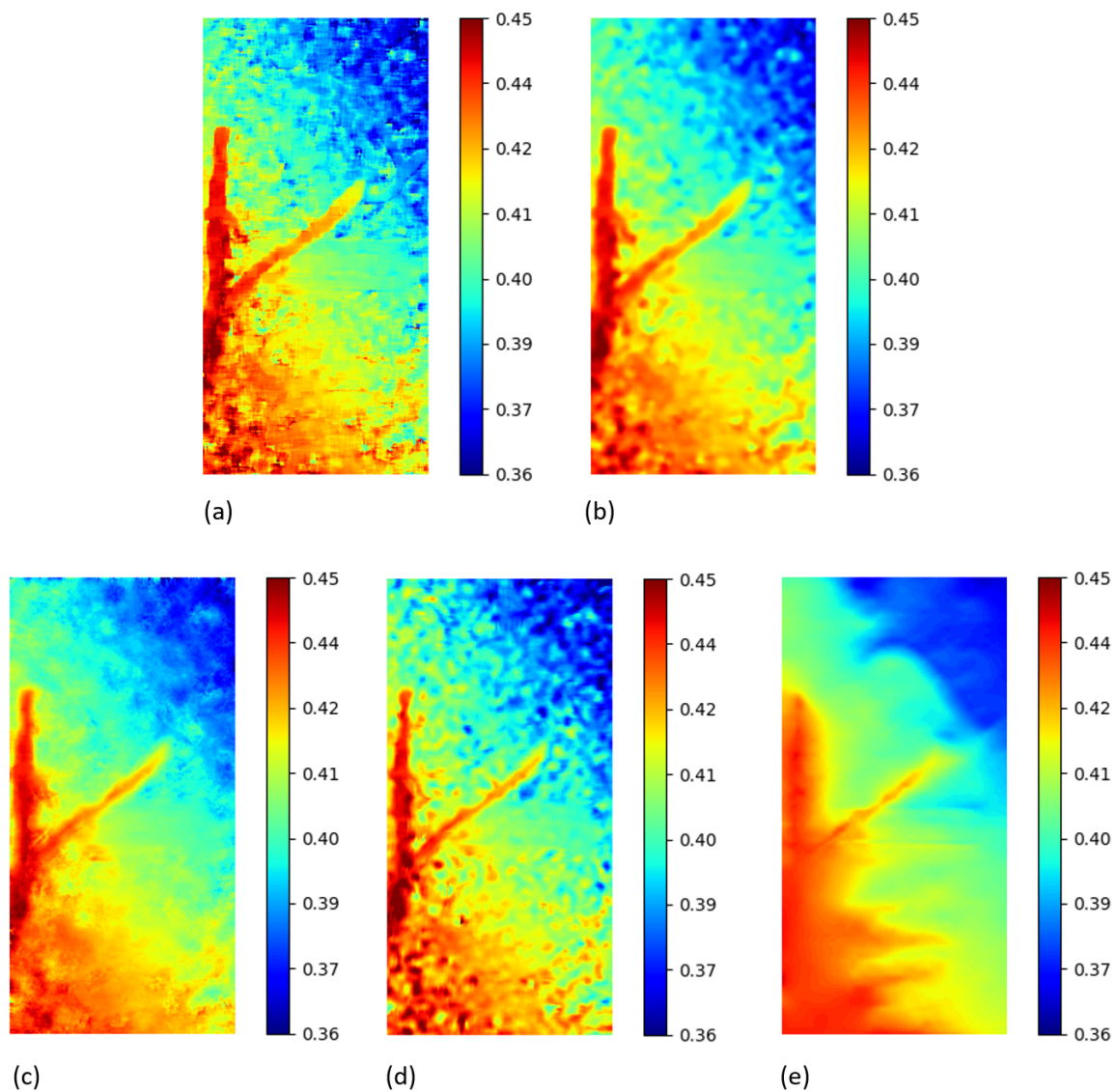
Figure 11. v displacements (mm) for the tensile test of GFRP sample obtained from DIC technique. (a) py2DIC raw results (b) py2DIC smoothed results using Gaussian filter (c) Ncorr results (d) Vic-2D results (e) DICE results [11].
