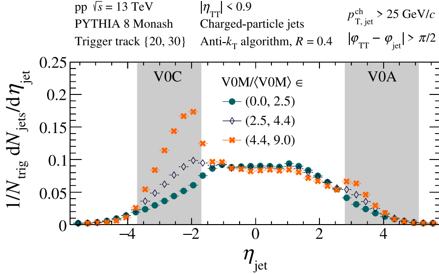
Figure 5. Same as figure 4, but for recoil jets with p_{\text{T, jet}}^{\text{ch}} > 25 GeV/c for various intervals in \text{V0M}/\langle \text{V0M} \rangle . Distributions are normalized per trigger.
