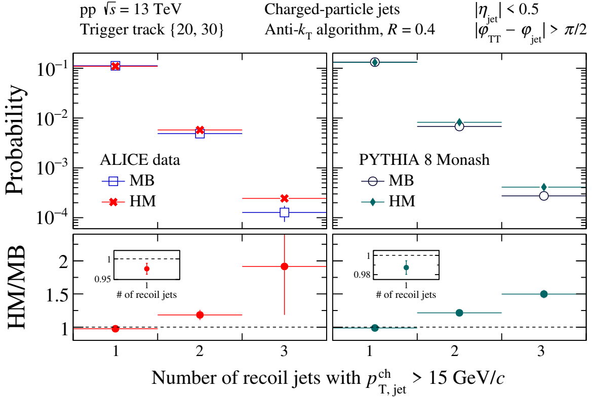
Figure 6. Distribution of probability per trigger hadron of number of jets with R = 0.4 and p_{T,\text{jet}}^{\text{ch}} > 15 \text{ GeV}/c recoiling from a high- p_T hadron (TT{20,30}) at midrapidity ( |\eta_{\text{jet}}| < 0.5 ), for MB and HM pp collisions at \sqrt{s} = 13 \text{ TeV} . Left panels: ALICE data; right panels: simulations at the particle level with PYTHIA 8 Monash tune. Lower panels show the ratio HM/MB. The insert in the lower panels has magnified vertical scale to show the ratio of probabilities to observe a single jet.
