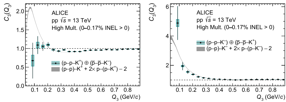
Fig. 2 Correlation functions (data points) for p–p–K + (left panel) and p–p–K – (right panel) compared to the lower-order contributions evaluated using the projector method (grey bands). Statistical and systematic uncertainties are represented by error bars and green boxes, respectively.
