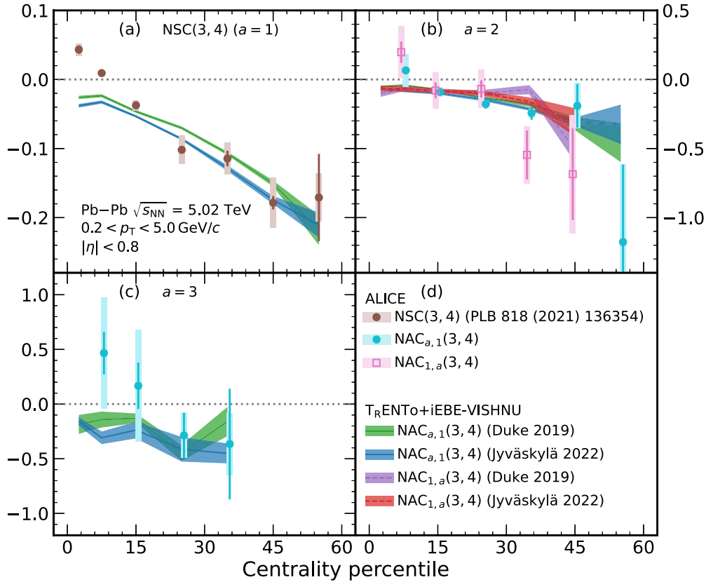
FIG. 4. Centrality dependence of the different orders a = 1, \dots, 3 of \text{NAC}_{a,1}(3, 4) (cyan closed circles) and \text{NAC}_{1,a}(3, 4) (pink open squares) compared with the theoretical predictions from \text{T}_\text{R} \text{ENTo} + \text{iEBE-VISHNU} for the Duke 2019 [22] and Jyväskylä 2022 [12] parametrizations. The statistical uncertainties in the calculations are indicated by the thicknesses of the colored bands. The data points for \text{NSC}(3, 4) are taken from Ref. [17].
