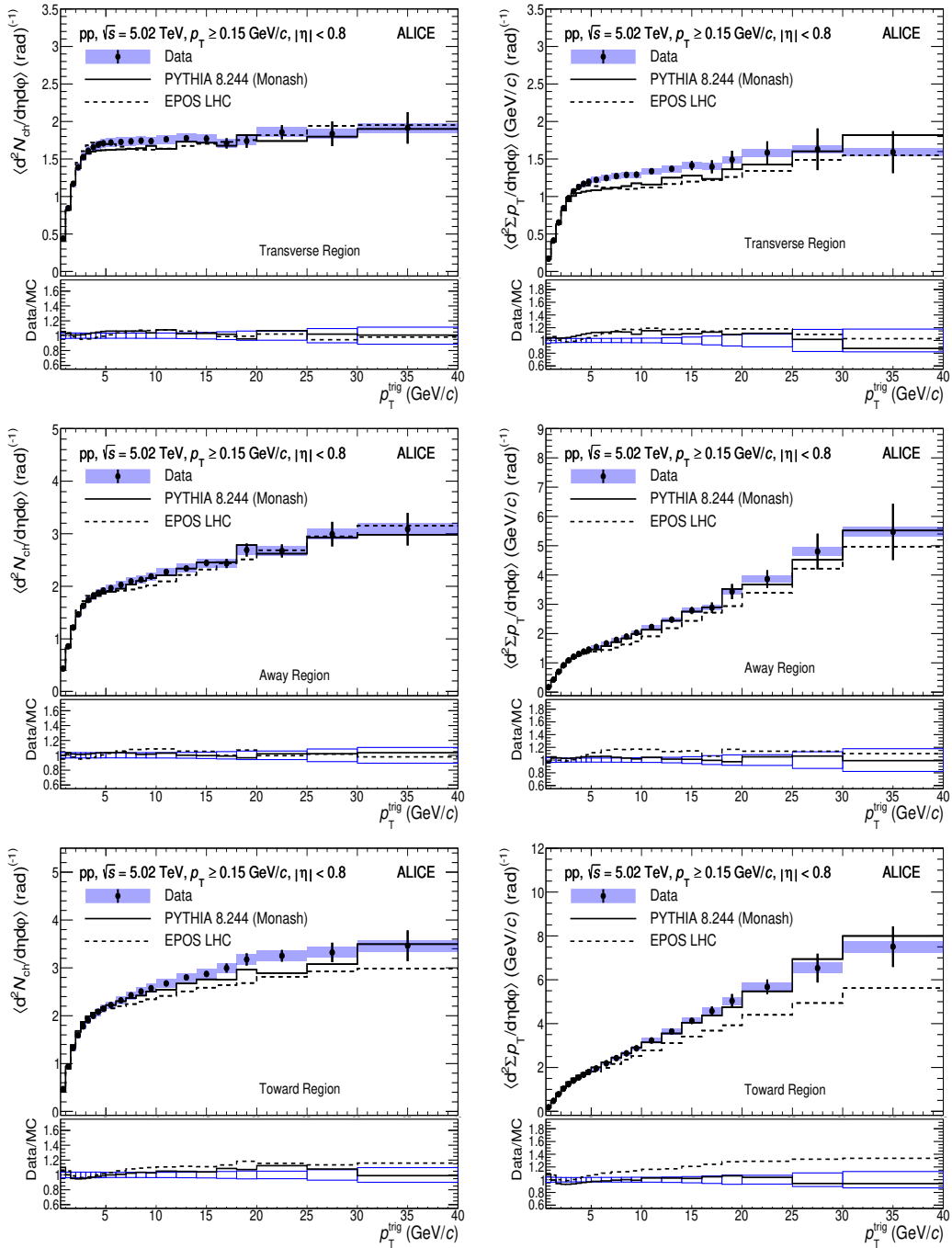
Figure 10. The charged-particle number (left) and summed- p_T (right) densities as a function of p_T^{\text{trig}} in pp collision at \sqrt{s} = 5.02 TeV are displayed. Results for the transverse (top), away (middle), and toward (bottom) regions were obtained for the transverse momentum threshold p_T > 0.15 GeV/c. The shaded area and the error bars around the data points represent the systematic and statistical uncertainties, respectively. Data are compared with PYTHIA 8/Monash (solid line) and EPOS LHC (dashed line) predictions. The data-to-model ratios are displayed in the bottom panel of each plot. The boxes around unity represent the statistical and systematic uncertainties added in quadrature.
