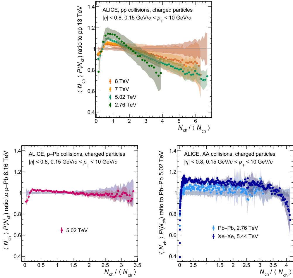
Fig. 5. Ratios of the KNO-scaled multiplicity distributions at various centre-of-mass energies per nucleon pair relative to \sqrt{s} = 13 \text{ TeV} for pp collisions (top panel) and relative to \sqrt{s_{NN}} = 8.16 \text{ TeV} and \sqrt{s_{NN}} = 5.02 \text{ TeV} for p-Pb and Pb-Pb collisions, respectively (left and right bottom panels). Statistical and systematic uncertainties are shown as bars and semi-transparent bands, respectively.
