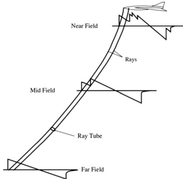
Figure 1: Sonic boom propagation through the atmosphere
