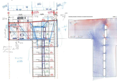
Fig. 4. Comparison of bidimensional analysis with software Cedrus stress-fields
