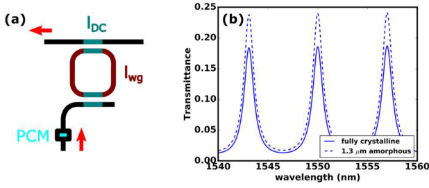
Fig. 5. Synapse simulation, (a) Part of the neuro-synaptic system that comprises the synapse. The arrows represent the input and output ports in the simulation. (b) Calculated transmittance of a synapse in its fully crystalline state (solid line) and a partially amorphous state, specifically for z_{\text{int}} at 1.3 \mu\text{m} (dotted line).
