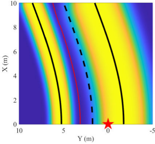
FIGURE 4. Example of lane change PF built to move on the left line. The red star represents the vehicle position, the black lines are the lane boundaries and the red line is the minimum APF value within the road boundaries.
