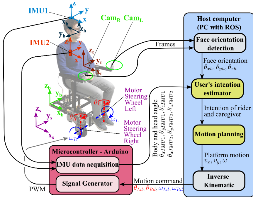
Fig. 1 Hand-free wheelchair working principle.
