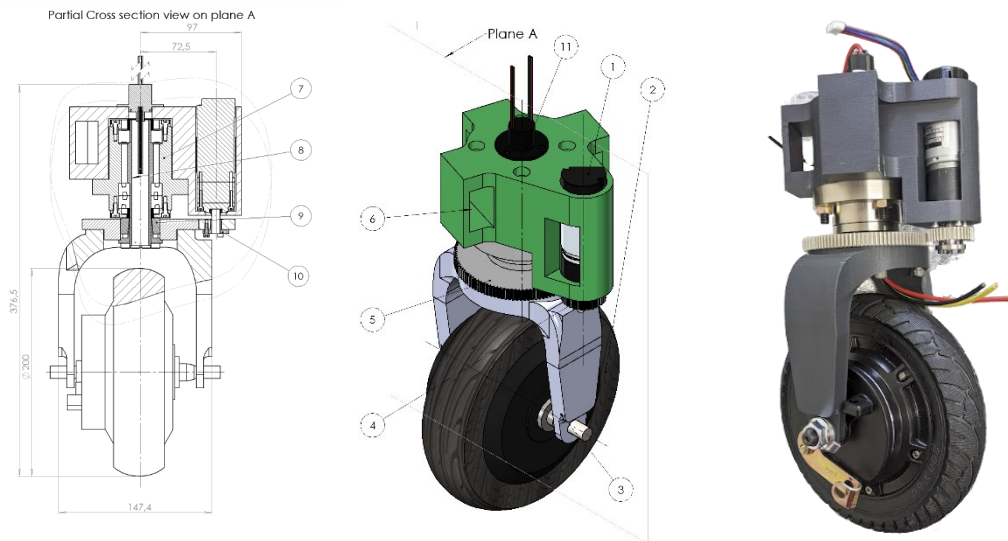
Fig. 3 Design of the motor steering wheel module (L, M) and developed prototype (R).
