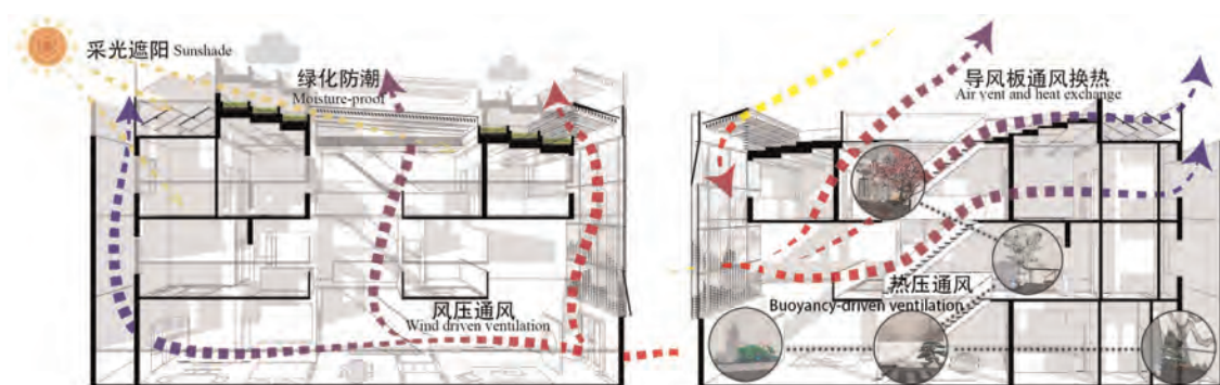
Figure 14. Indoor ventilation.
