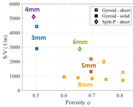
Fig. 2. Surface-to-fluid volume ratio versus porosity for the TPMS adopted in the mirror cooling. Different colors correspond to different values of L_c .
