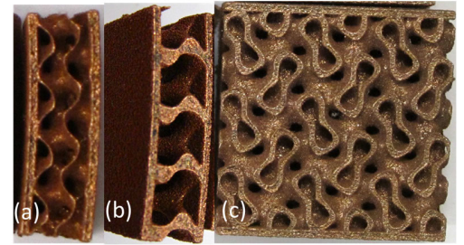
Fig. 1. Picture of a (a) sheet gyroid, (b) solid gyroid, and (c) sheet Split-P realized in CuCrZr by AM at the INFN premises in Padua, using laser powder bed fusion.
