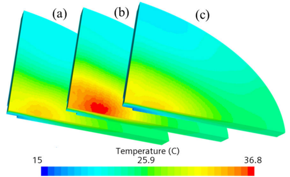
Fig. 8. Temperature map for (a) GX1, (b) GY2, and (c) SX1.
