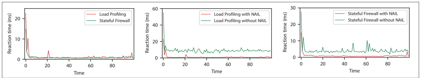
FIGURE 4. a) Reaction time when an update() is requested for a load profiling and a stateful firewall application; b) Comparing the reaction time when an update() is performed with NAIL and without NAIL for a load profiling; c) For a stateful firewall.
