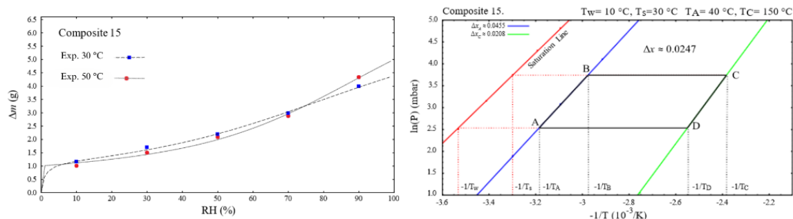
Figure 2. On the left, experimental adsorption isotherms at 30 °C and 50 °C for composite 15, with the related fitting curve. On the right, charging/discharging thermodynamic cycle for the same composite with the operational boundaries that are average winter temperature ( T_w ), average summer hot temperature ( T_s ), user operating temperature ( T_A ) and heat source temperature ( T_C ).
