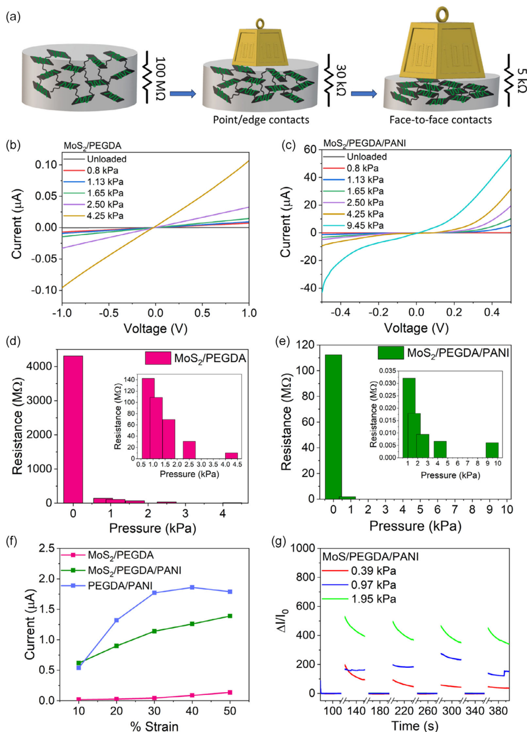
Figure 4. Evaluation of the piezoresistive behavior of hybrid hydrogels. a) Schematic illustration of the piezoresistive sensing mechanism with the increase of external pressure. b,c) I - V characteristics and d,e) resistance trends of, respectively, \text{MoS}_2/\text{PEGDA} and \text{MoS}_2/\text{PEGDA}/\text{PANI} free-standing hydrogels as a function of the applied pressure (weights displaced on top of the gel surface and current measured at the bottom by disposing the samples on gold electrode substrates). f) Current-strain curves for the three samples and g) chronoamperometric data for \text{MoS}_2/\text{PEGDA}/\text{PANI} hydrogel.
