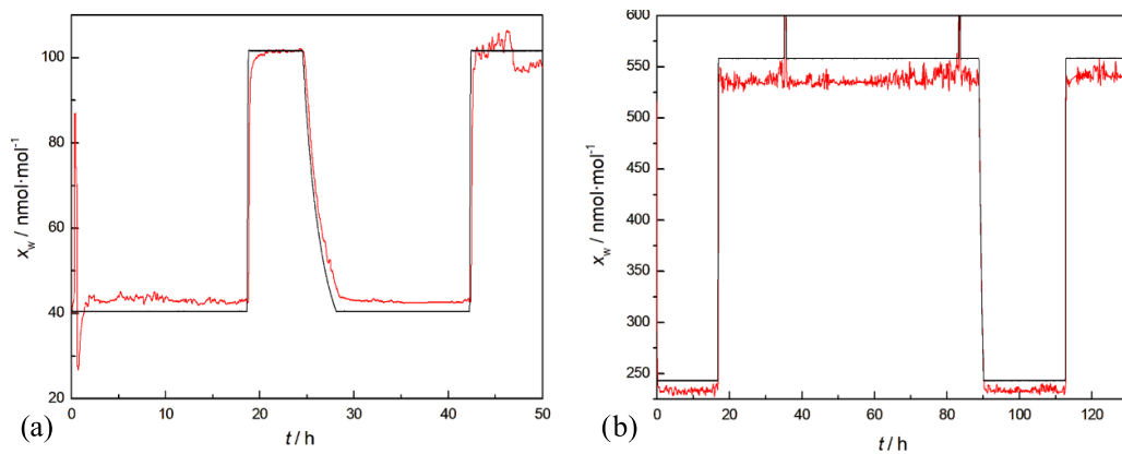
Figure 8. Response of the humidity generator at step changes of the saturation temperature; (a) between -95^{\circ}\text{C} and -90^{\circ}\text{C} (that is, between 40 and 100 ppb) and (b) between -85^{\circ}\text{C} and -80^{\circ}\text{C} (that is, between 240 ppb and 550 ppb). Measurements have been carried out at 2 \text{ l}\cdot\text{min}^{-1} at a pressure of 1000 hPa. The red line represents the water vapour amount fraction measured by the CRDS, x_{w,CRDS} ; the black line represents the reference water vapour amount fraction x_{w,0} estimated from the measurement of T_{sat} and p .
