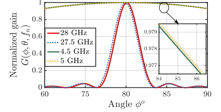
Figure 4: Illustration of beam squinting effects at 5GHz and 28GHz with N_t^{5GHz} = 2 , N_t^{28GHz} = 32 , and steering angle = 80^\circ .
