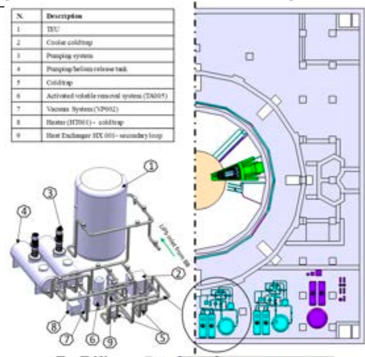
Figure 26. TER integration into the tokamak building.
