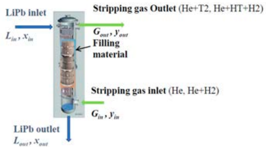
Figure 10. Sketch of the GLC extractor with the nomenclature of the efficiency calculations. The most relevant results obtained in TRIEX-II were achieved by solubilizing deuterium in liquid LiPb and extracting it with a stripping gas of helium plus a 0.5% vol. addition of hydrogen in order to enhance the extraction efficiency. The results of the 6 tests are reported in Figure 11. The picture shows the extraction efficiency as a function of the L/G ratio, expressed as \text{m}^3/\text{m}^3 , i.e. the ratio between the liquid LiPb mass flow rate and the stripping gas flow rate. The former flow rate was varied in the range of 0.5–1 kg/s and the latter in the range of 10–100 l/h, with a LiPb temperature of 450^\circ\text{C} . As detailed in [7], the extraction efficiency was measured by means of a quadrupole mass spectrometer, calibrated such that the isobaric interferences were reduced as low as possible, enabling the possibility to discern \text{D}_2 from He. The maximum extraction efficiency rate of 44% was found for an
