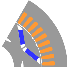
Fig. 7. Radial cross-section of the Tesla Model 3 PMSM.
