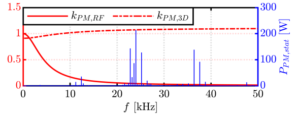
Fig. 8. PM loss harmonics according to the magnetostatic solution of FEMM and the correction factors to account for the reaction field and the 3D effects. The results refer to OP#1.
