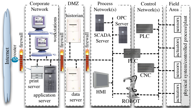
Fig. 1. Typical connections of IACS to corporate networks and the Internet
