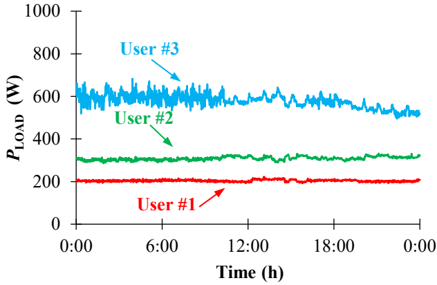
Fig. 6. Load power profiles on 2023, January 28 th for the three users.
