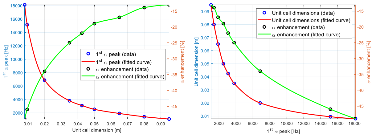
Figure 1: Absorption coefficient design curves as a function of the unit cell dimension (on the left) and the frequency of the 1 st peak (on the right).
