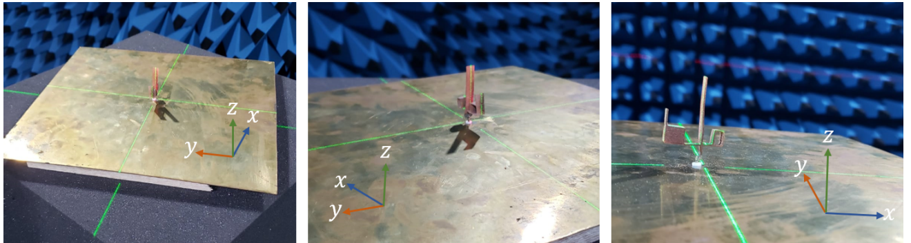
Figure 4. Measurement setup.
