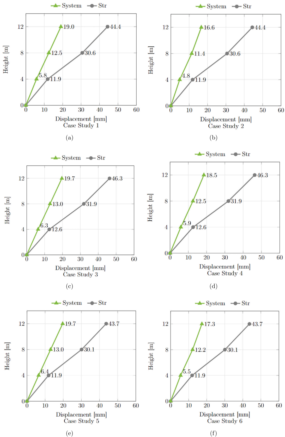
Fig. 9. Floor displacements before (Str) and after (System) the retrofitting intervention for each Case Study (CS#).
