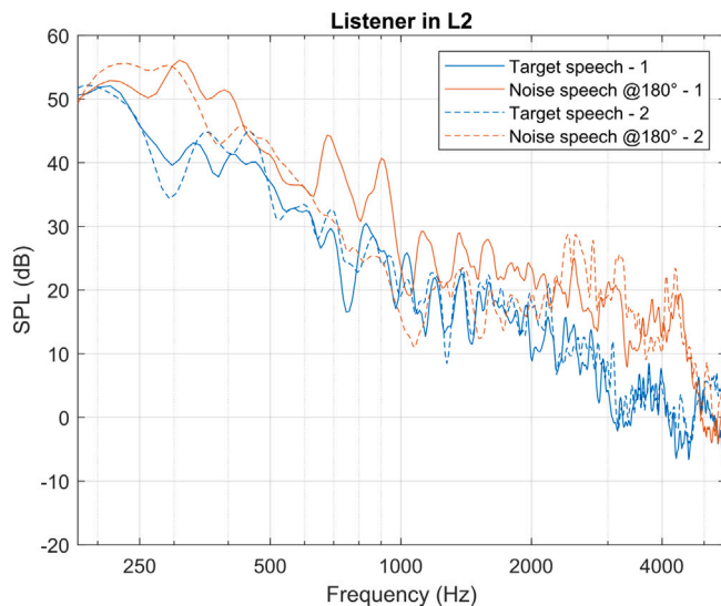
Fig. 7. Examples of auralized target and noise speech spectra with 5 dB SNR for the scene with the listener in L2 location and noise at 180^\circ azimuth.
