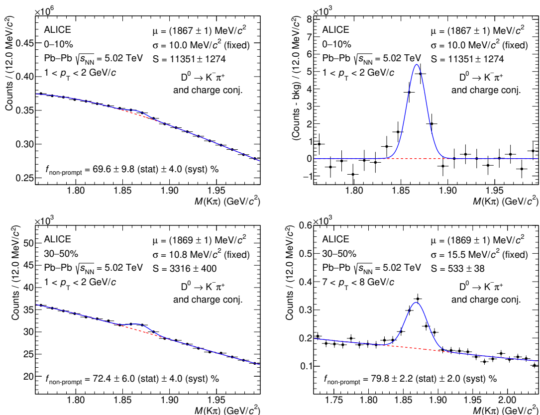
Figure 1. Invariant-mass distributions for D^0 candidates in selected p_{\text{T}} intervals for the centrality class 0–10% and 30–50%. Fitted values for the D^0 meson mass \mu , width \sigma , and raw yield S are also given, the fraction of D^0 candidates in the measured raw yield is reported with its statistical and systematic uncertainties. Top row: non-prompt D^0 mesons with 1 < p_{\text{T}} < 2 \text{ GeV}/c in the 0–10% centrality class, before (left) and after (right) subtraction of the background fit function. Bottom row: non-prompt D^0 mesons with 1 < p_{\text{T}} < 2 \text{ GeV}/c (left) and 7 < p_{\text{T}} < 8 \text{ GeV}/c (right) in the 30–50% centrality class.
