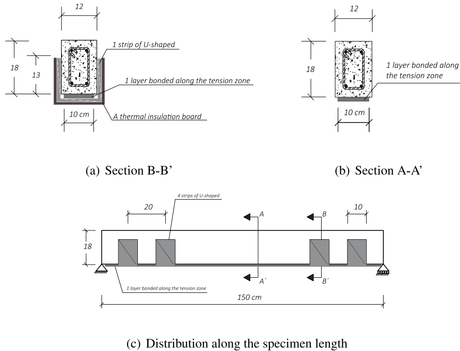
Fig. 4. CFRP schemes.
