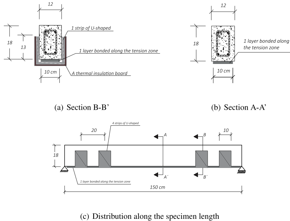
Fig. 4. CFRP schemes.
