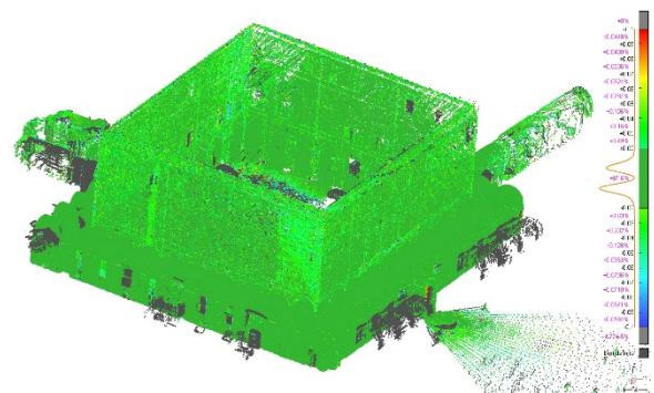
Figure 14. Cloud-to-cloud discrepancy analysis between MMS data and Flash data.
