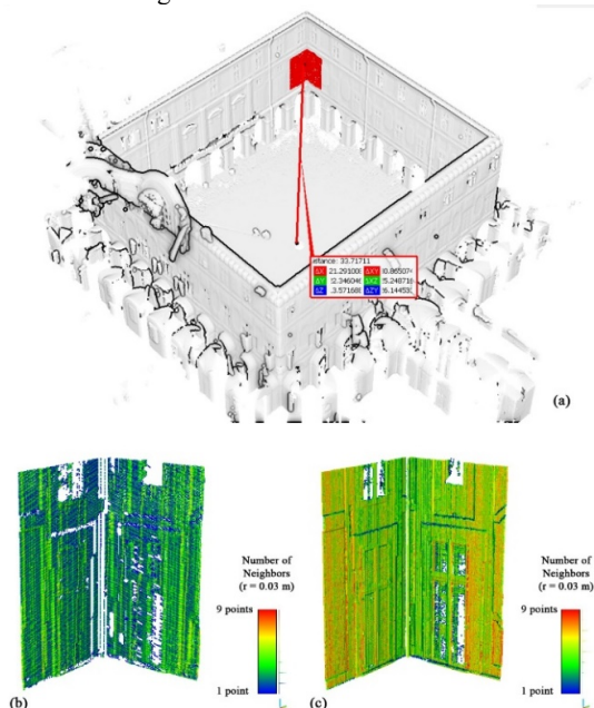
Figure 8. (a) Position of analysed surfaces (b) Detail of the density analyses carried out on the Flash scan acquired in the center of the cloister; (c) the density analyses carried out on the traditional static scan acquired in the center of the cloister.
