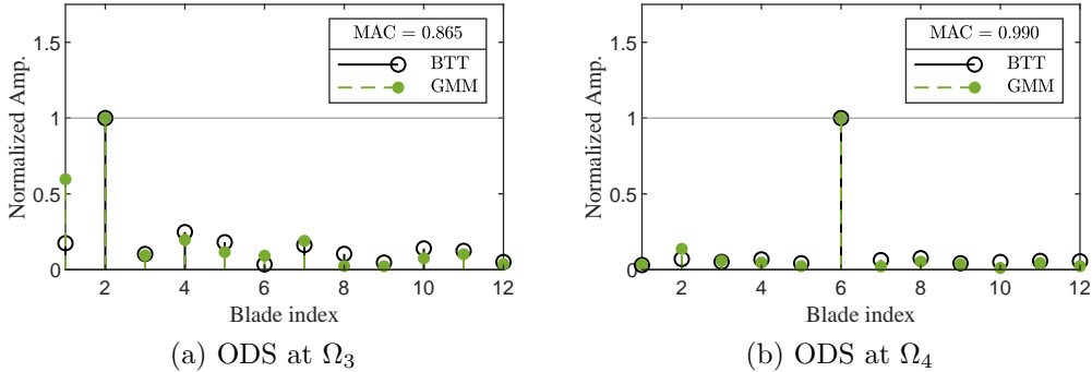
Figure 17: Comparison of tested/BTT measured and GMM predicted ODS at 1T mode/EO20 resonance in the spinning rig test.
