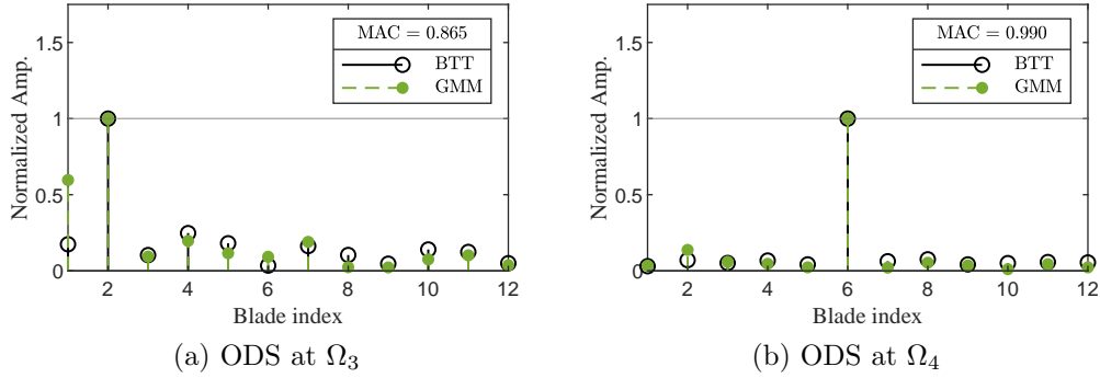
Figure 17: Comparison of tested/BTT and GMM predicted ODS at 1T mode/EO20 resonance in the spinning rig test.
