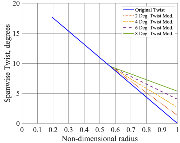
Fig. 12 Modifications to the blade twist rate for different collective angles assessed
