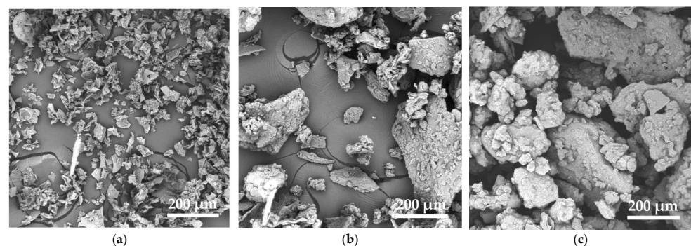
Figure 2. SEM micrographs of three different bio-fillers: (a) wine lees (WL), (b) grape pomace (GP) and (c) grape seeds (GS).
