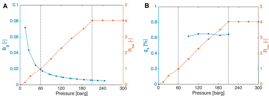
FIGURE 7 Scenario of pure H 2 in brine 1 at 45°C: (A) R sw and B g ; (B) percentage of gas in solution.
