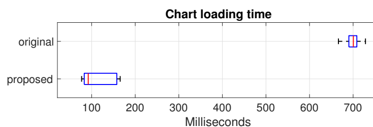
Figure 17. Loading time comparison between the proposed implementation and the original one, provided as a default by Grafana, for updating a chart embedded in an iframe . On each box, the central mark indicates the median, the bottom and top edges of the box indicate the 25th and 75th percentiles, respectively, and the whiskers extend to the most extreme data points, the minimum and the maximum values.
