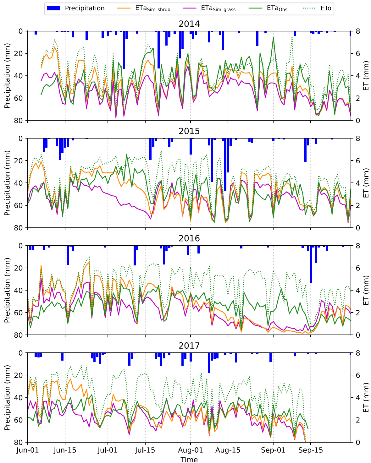
Fig. 7. Daily time series of actual evapotranspiration from eddy covariance ( ET_{aObs} ), modeled actual evapotranspiration from single vegetation simulations ( ET_{aSim} grass, ET_{aSim} shrub), potential evapotranspiration ( ET_0 ) and precipitation for the four analyzed growing seasons.
