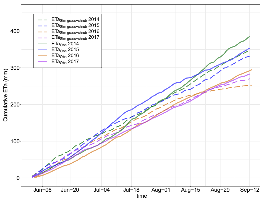
Fig. 5. Cumulative actual evapotranspiration as modeled by Hydrus 1D double vegetation (“grass + shrub”, mixture of grassland and shrubland) and from eddy covariance measures.
