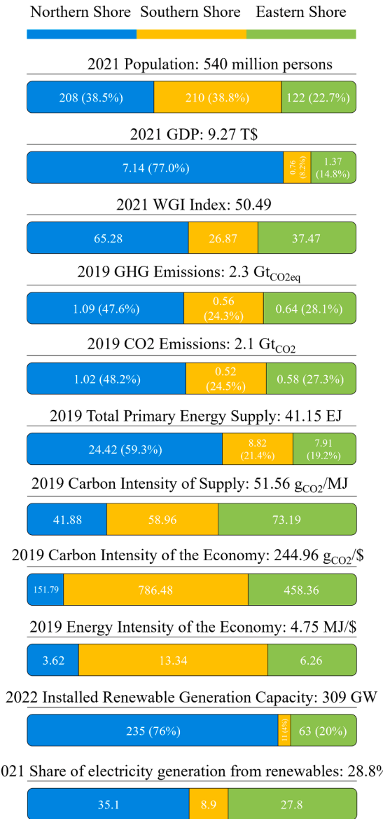
Fig. 1. Graphical characterization of the Mediterranean basin.
