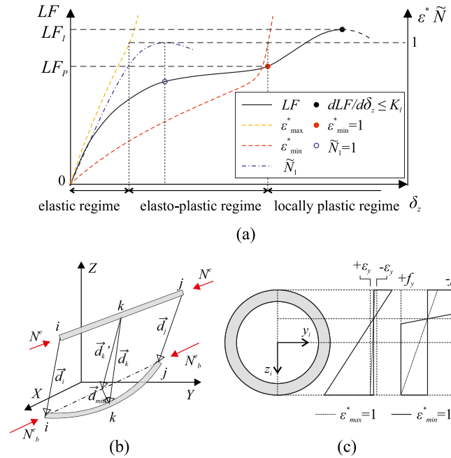
Fig. 2. Structural performance: Conceptual graphical scheme exemplifying the variables used for establishing the critical load factor \hat{L}\hat{F} as the minimum between LF_I and LF_P (a), the member buckling (b, after [68]), and the member cross-section yielding (c).
