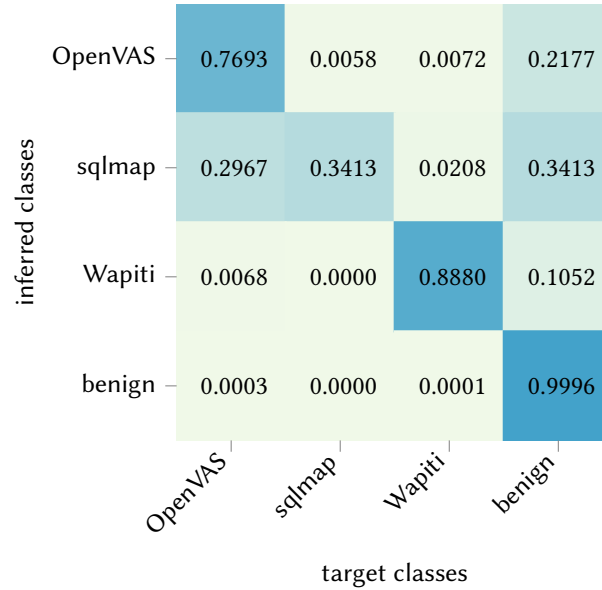
Figure 1: Normalized confusion matrix of our random forest.
