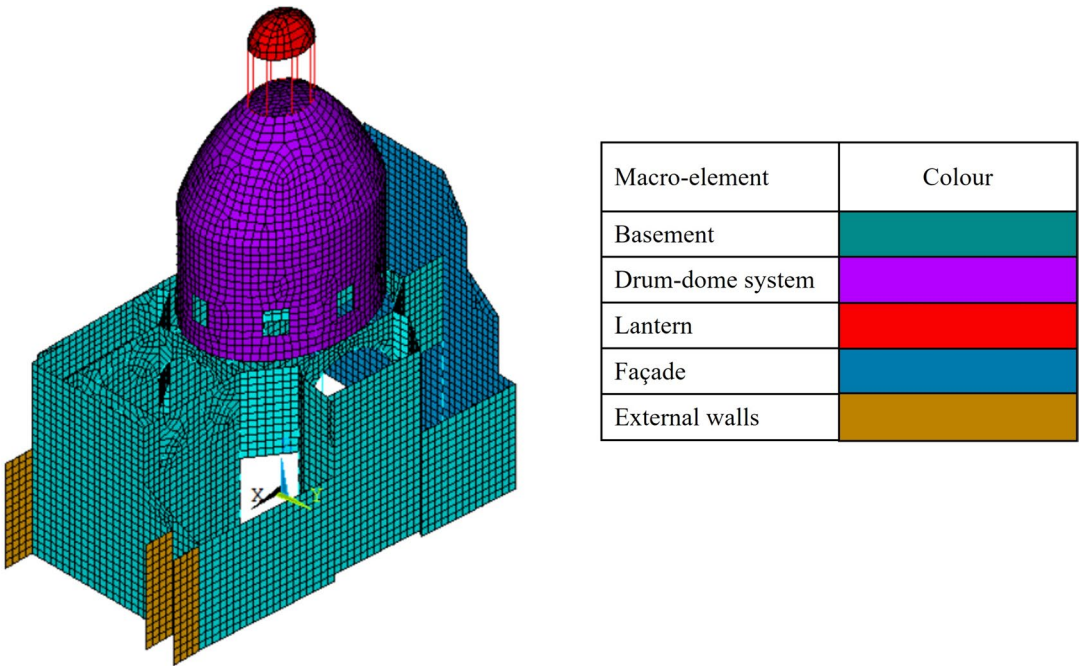
Fig. 3 Mechanical model of the Church of Santa Caterina with related macro-elements
