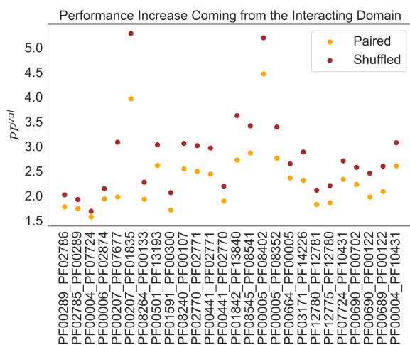
Figure 3. Performance (lower better) increases when taking domain sequence in context into account. We plot the perplexity \mathcal{P}^{val} for target sequences on the validation set, once for a shallow Transformer trained with the true pairings (Paired) and once for a shallow Transformer trained with shuffled pairs in the training set. (“Paired” is always below “Shuffled” with an average difference of 0.48).
