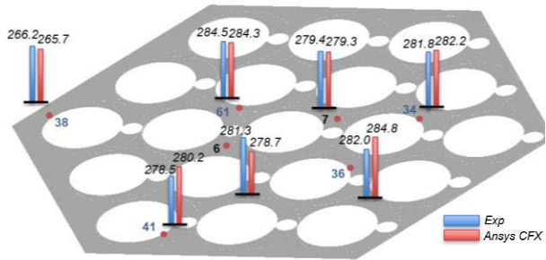
Figure 5. TCs temperature comparison on Plane 2
