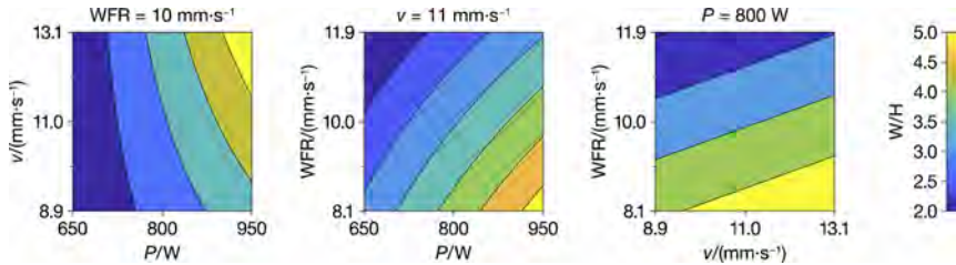
Figure 14 W/H contour plots at P = 800 W, v = 11 mm·s -1 , and WFR = 10 mm·s -1 (see online version for colours)
