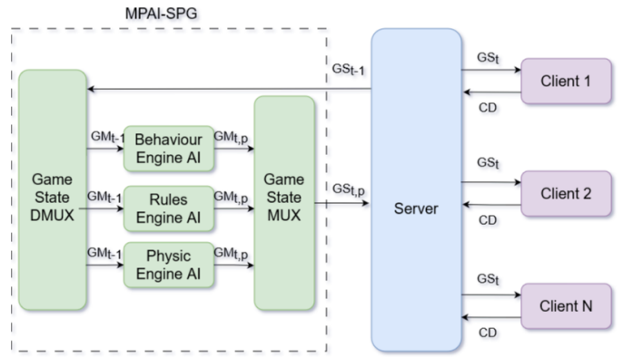
Fig. 1. MPAI-SPG architecture
