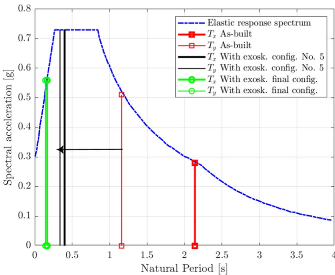
Fig. 17 Elastic response spectrum indicating the fundamental period in the x direction before and after retrofiting
