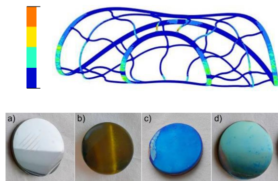
Figure 1. A: Maximum Principal Strain reached by the implant during bending. B: Polished Ø25 mm nitinol disks (56.0 wt% Ni, A_f = -14.1^\circ\text{C} ) a) as-polished, b) after heat-treatment at 400°C, c) 450°C and d) 500°C.
